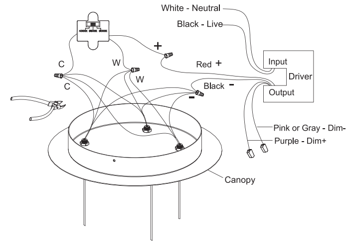
Fig. 2 Wire Diagram
